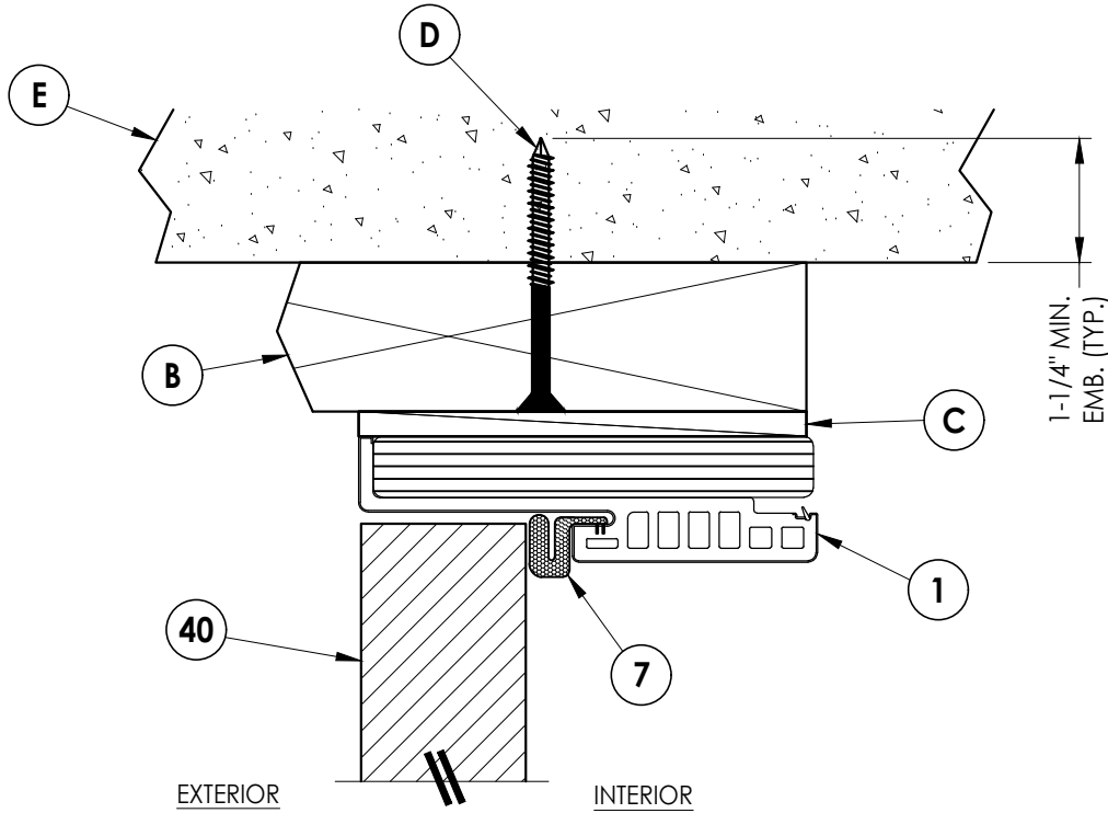
1 VERTICAL CROSS SECTION 3 2X Buck Construction - Single Door Only Outswing Shown (Inswing Similar)
