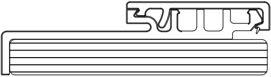
SIDE JAMB (2-PIECE)
