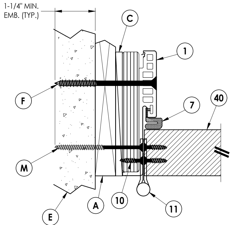
3 HORIZONTAL CROSS SECTION 4 1X Buck Construction Outswing Shown (Inswing Similar)
