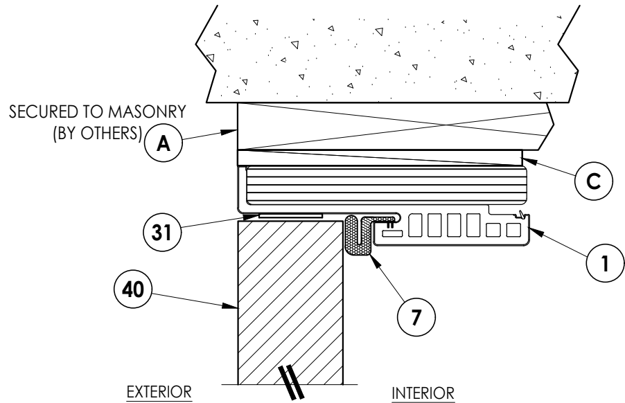
1 VERTICAL CROSS SECTION 4 2X Buck Construction - Single Door Only Outswing Shown (Inswing Similar)
