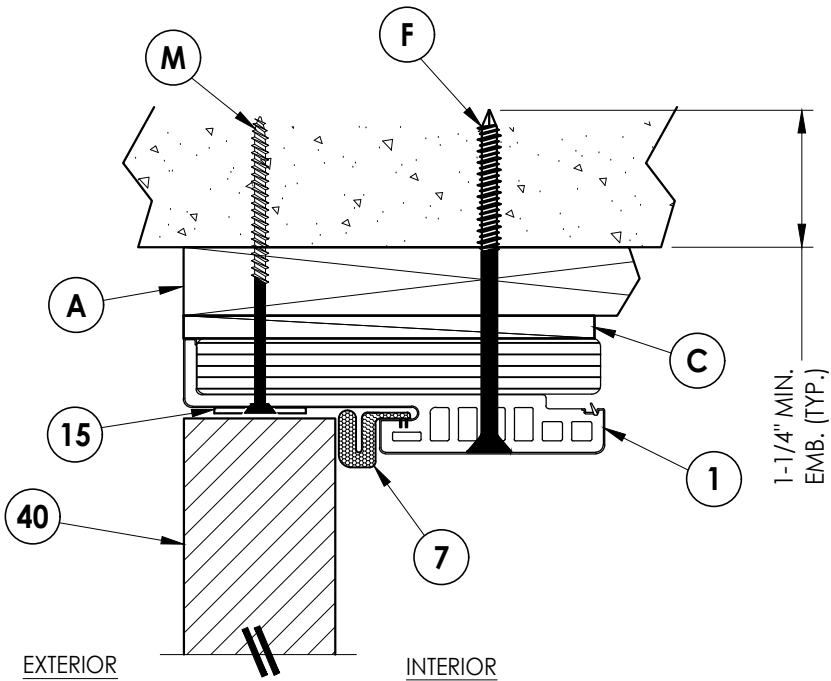
2 VERTICAL CROSS SECTION 4 1X Buck Construction - Double Door Outswing Shown (Inswing Similar)
