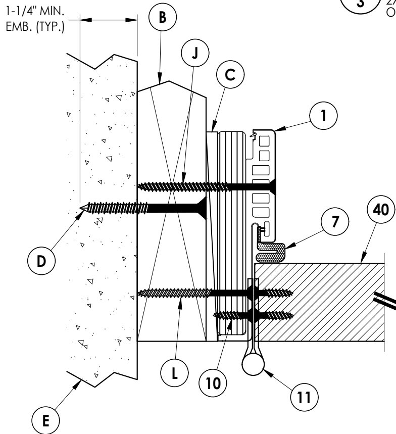
3 HORIZONTAL CROSS SECTION 3 2X Buck Construction Outswing Shown (Inswing Similar)
