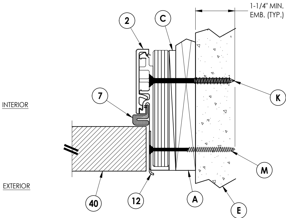
4 HORIZONTAL CROSS SECTION 4 1X Buck Construction Outswing Shown (Inswing Similar)
